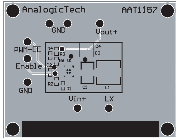
Figure 3: AAT1157 Evaluation Board Bottom Side.
