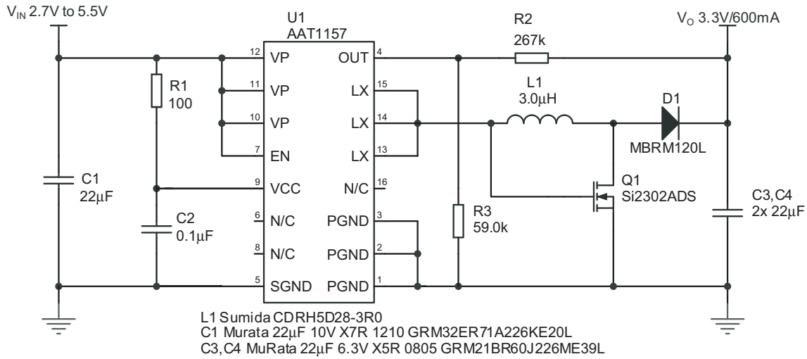
Figure 4: AAT1157 Buck Boost Converter.
